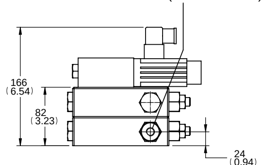
負載感應接口 Load-sensing port G 1/4 BSPP (threads code: 1) 7/16-20 UNF (threads code: 3) M12xP1.5 ISO 6149-1 (threads code: 7)
