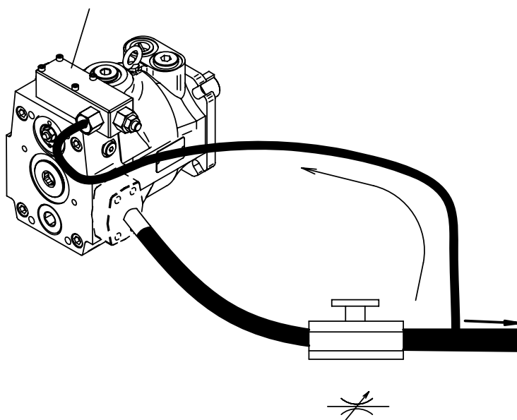
Load-sensing compensator
