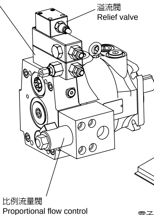
雙閥負載感應型調節器 Load-sensing compensator with NG6 interface
