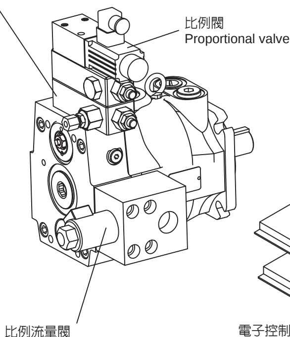
雙閥疊式負載感應型調節器 Load-sensing compensator with NG6 interface
