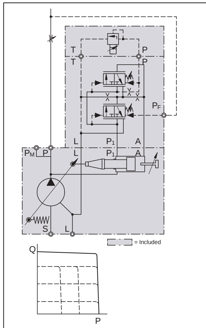
比例閥 Proportional valve
