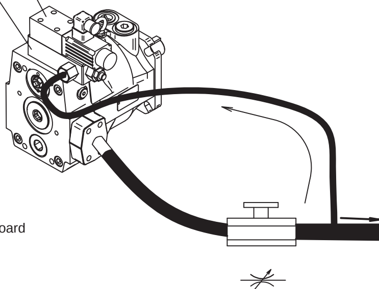
Proportional valve
