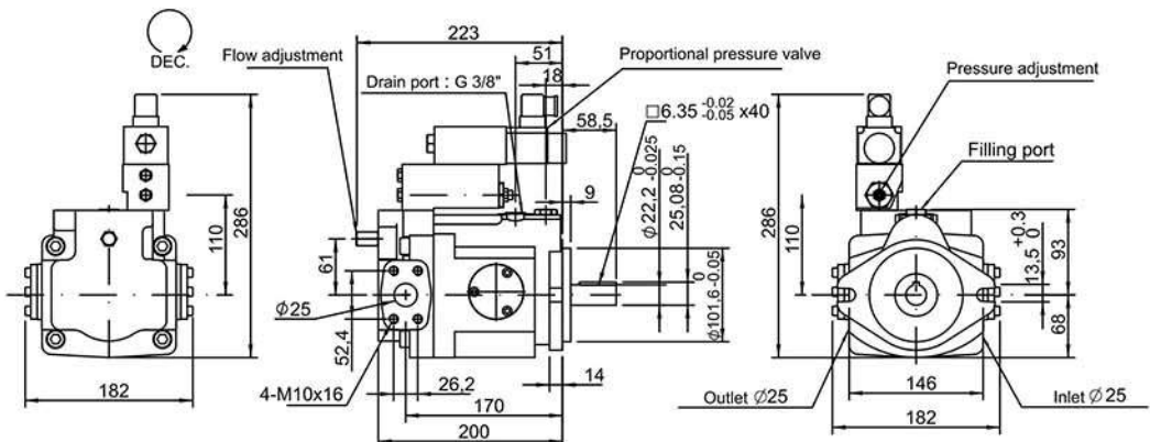
V23GJ, V25GJ Remote pressure compensator + Proportional pressure valve
