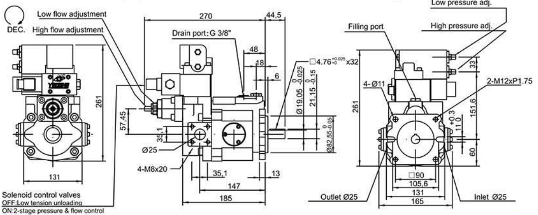
V15CR, V18CR 2-stage pressure &amp; Flow control + Low tension unloading
