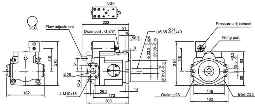
V23GM, V25GM Remote pressure compensator with NG6 interface
