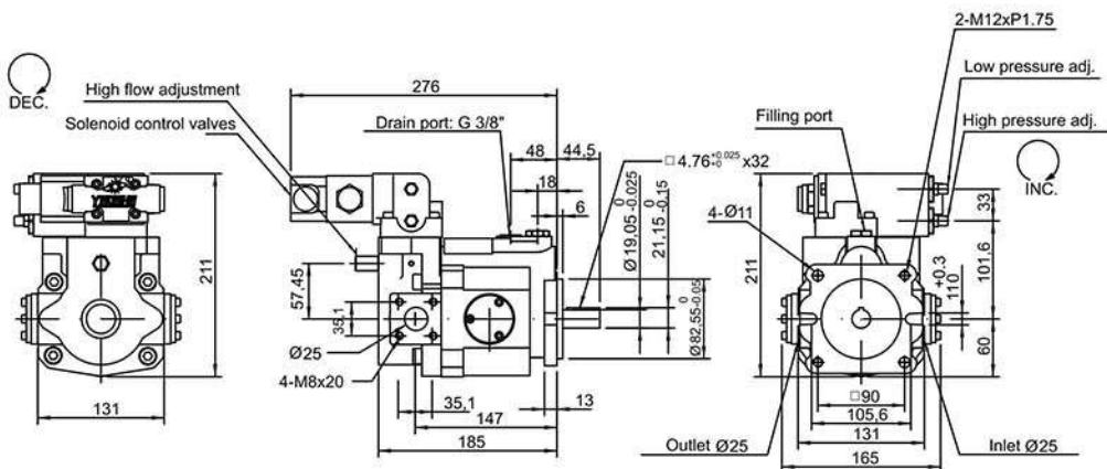
V15D, V18D Low tension unloading + Pressure control
