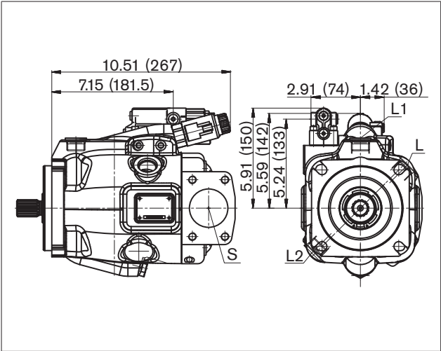
EP.ED / EK.ED Electro-proportional control, series 53
