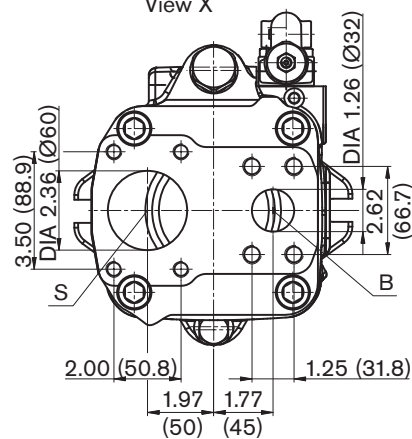
View X
