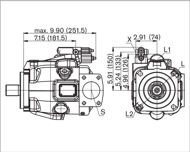
LA.D. Pressure, flow and power control, series 53
