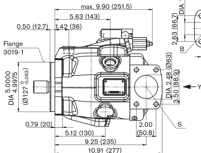
Detail Z
