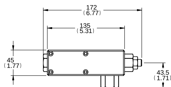
負載感應接□ Load-sensing port
